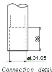
Connection detail
